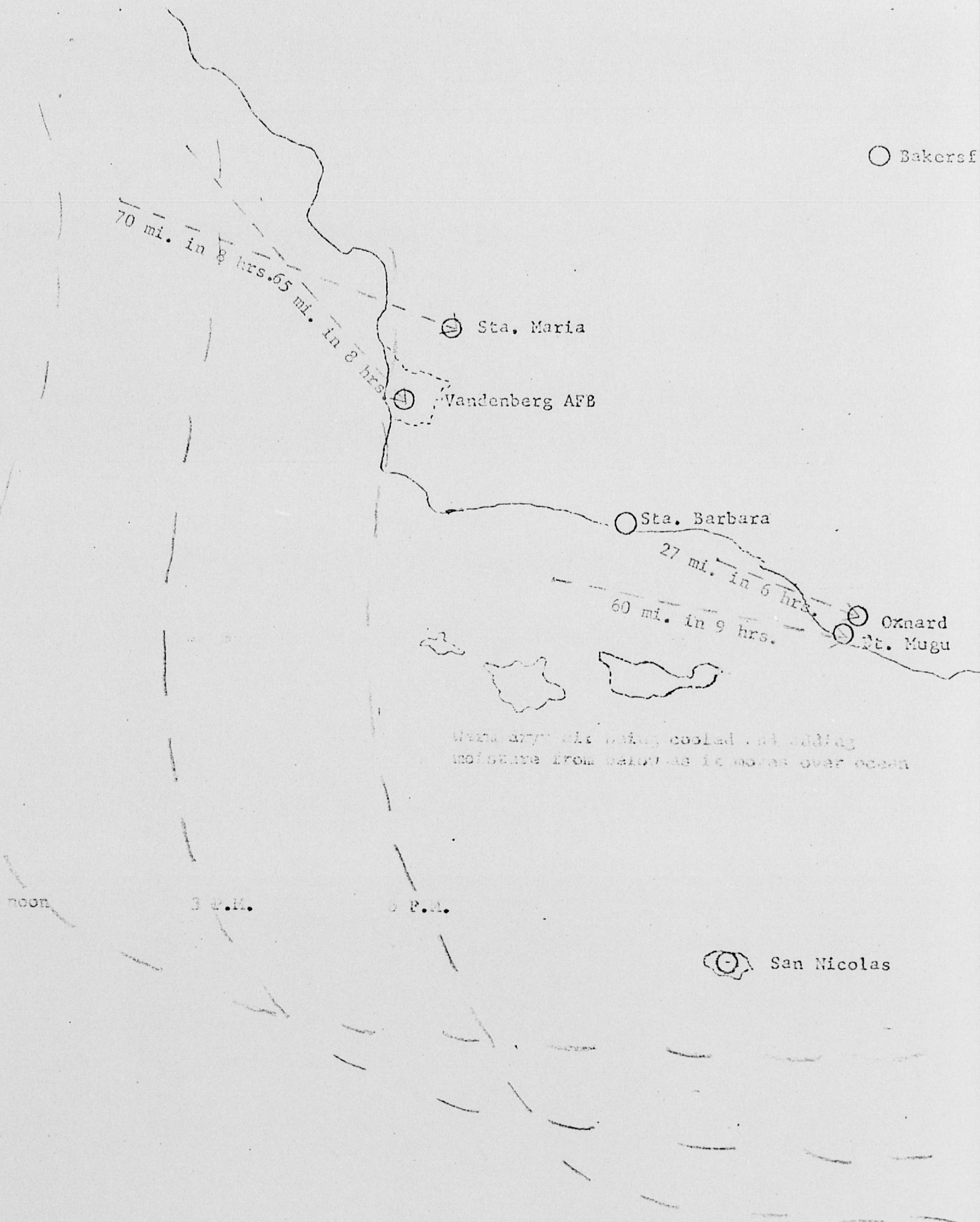
Fig. 2. Return Flow of Modified Air Arriving Over the Station From a Vector Path Between Noon and 8:20 P.M.
