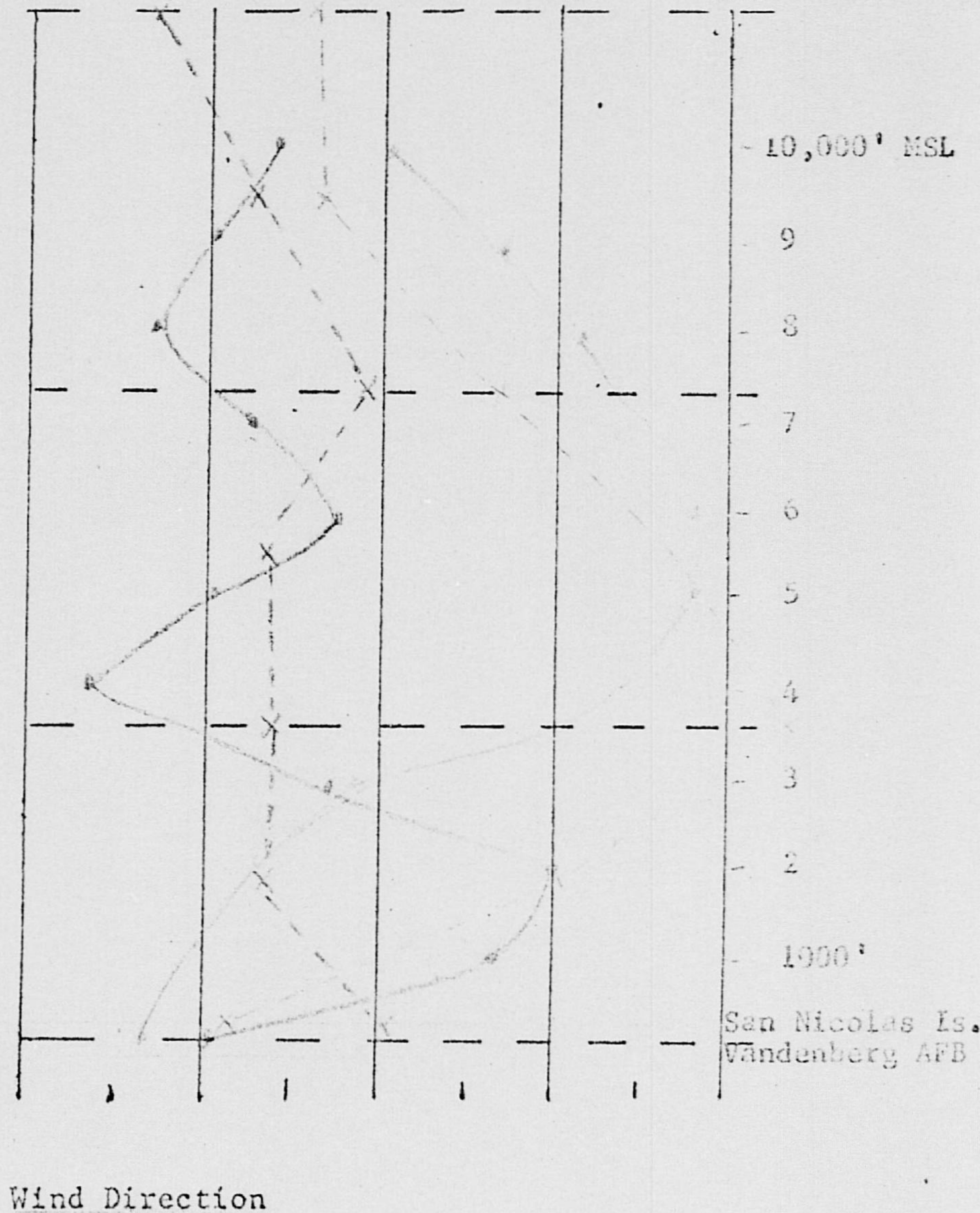
Fig. 4. Profiles of Temperature, Dew Point, Relative Humidity, Wind Direction and Velocity at Vandenberg AFB and San Nicolas Island during late Afternoon October 6, 1967.
